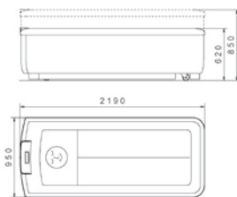
Lady-Spa dimensions standard cladding
