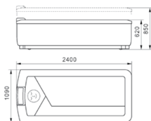
Thermo-Spa dimensions standard cladding
